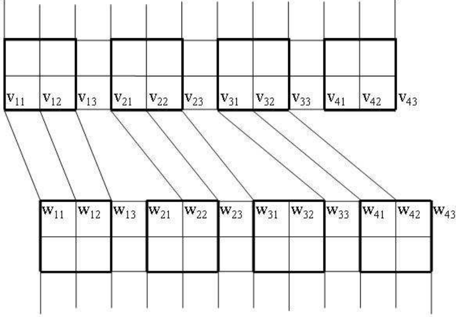
Figure 3: How to vertically connect two copies of B when d=2 .
