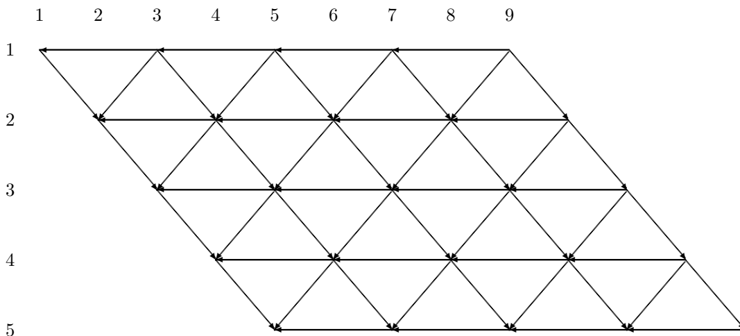
Figure 2: The triangle \mathcal{T}(5) .
