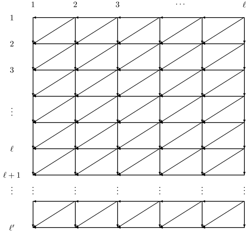
Figure 1: The admissible PDAG \mathcal{G}_{tri}(\ell', \ell) .
