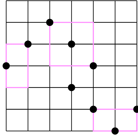
Figure 5: Different windows of nodes in a top-bottom minimal cutset of G_{sqr} .
