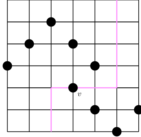
Figure 4: A unique path of v for the top-bottom minimal cutset.
