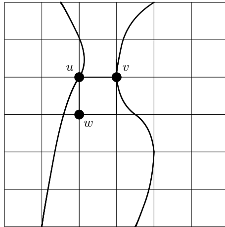
Figure 7: When some 1 \times 1 grid contains three points from a minimal cutset S .
