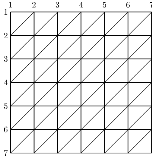
Figure 1: The grid G_{tri}(6, 6) .
