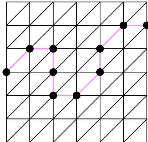
Figure 2: A restricted right-left NAW on G_{tri}(6, 6) and its corresponding top-bottom minimal cutset.
