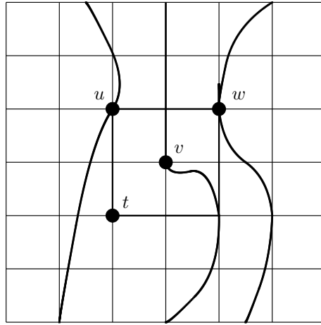
Figure 8: When some 2 \times 2 grid contains four points from a minimal cutset S .
