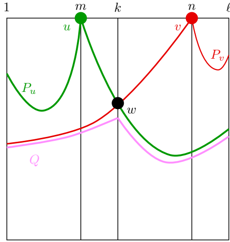
Figure 6: The path Q does not cross any node in S .
