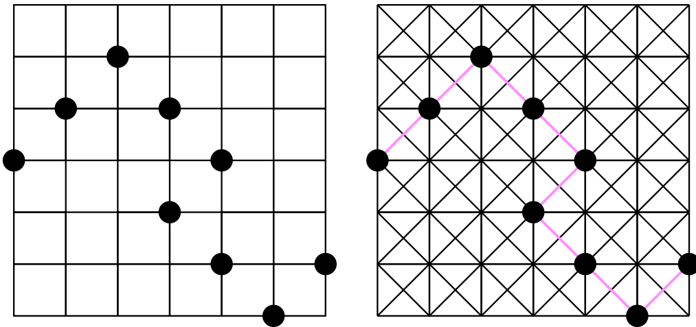
Figure 3: G_{sqr}(6, 6) and its corresponding G_{dia}(6, 6) . The node set presented in the graph is a minimal cutset of G_{sqr}(6, 6) . It is not a walk on G_{sqr} , but it is a NAW on G_{dia} .
